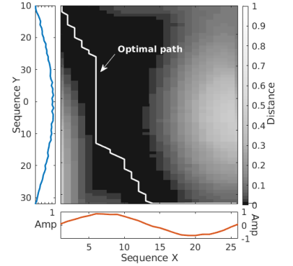
Fig. 5: DTW optimal alignment.
