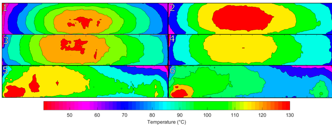
Figure 16. Greyscale method contour plots of the surface temperature profile measurements after each cycle of ablation using the Greyscale method.
