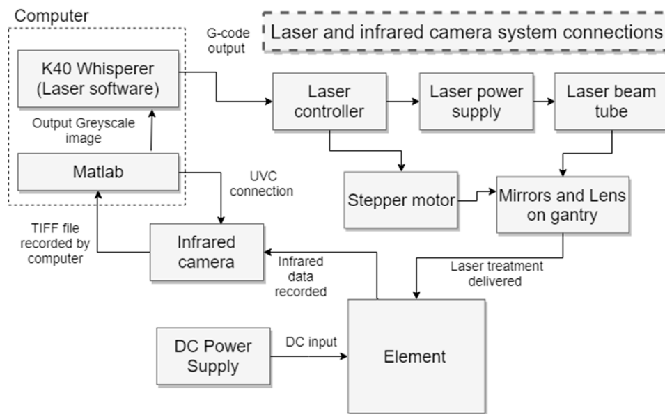
Figure 11. Connection of the components within the laser system.
