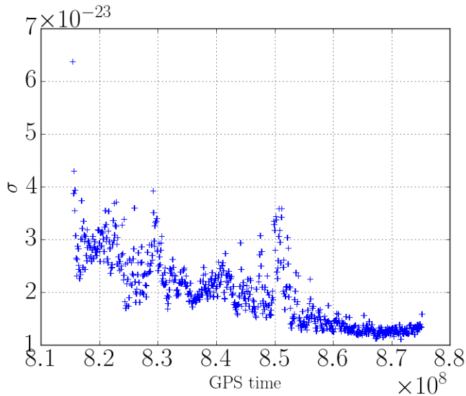
FIG. 5: Daily standard deviation of S5 H1 data heterodyned for the Crab pulsar (fig. 4).
