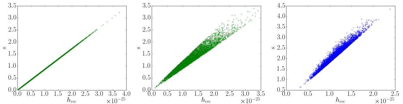
FIG. 6: Significance, eq. (42), vs. recovered strength, eq. (41), for searches over 5000 noise-only H1 S5 Crab instantiations using model-dependent eq. (43) (left), semi-dependent eq. (45) (center), and independent eq. (54) (right) templates. The model-dependent case assumes fully known \iota and \psi . Note that the number of degrees of freedom in the regression is manifested in the spread, which is due to noise: templates with a single degree of freedom are less susceptible to noise and the spread is minimal. The two plots on the left were generated using a GR template, but similar results are obtained for G4v.
