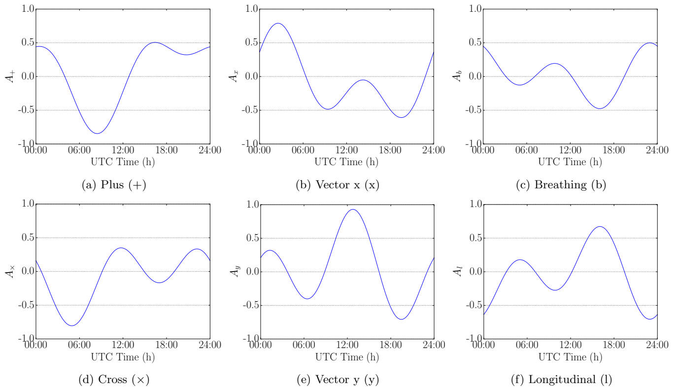
FIG. 2: LHO response A_p(t) , eq. (23), to different polarizations from the Crab (PSR J0534+2200), from 00:00 UTC to 24:00 UTC.
