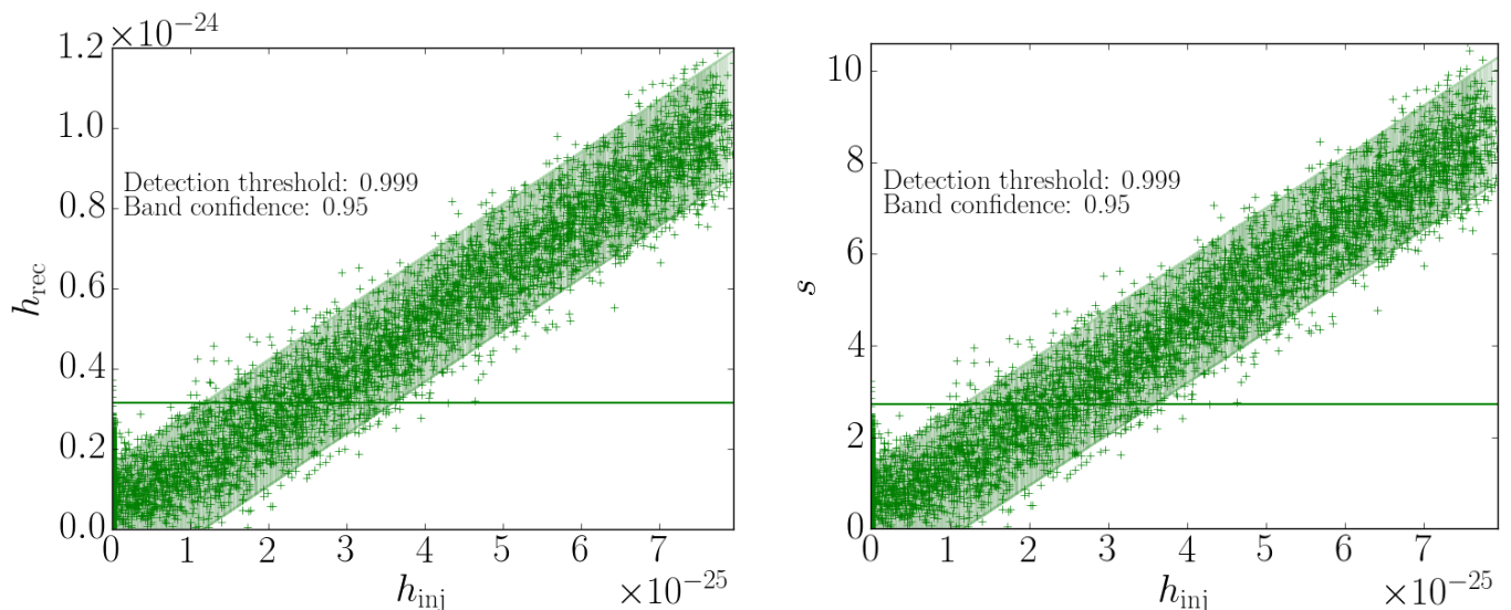
FIG. 8: Neyman plot of recovered signal strength h_{\text{rec}} (left) and significance s (right) vs. injected strength h_{\text{inj}} . In this case, GR signals are recovered with GR templates, but results are qualitatively the same with G4v injections recovered with G4v templates, or either kind of injection recovered with model-independent templates. The collection of points at h_{\text{inj}} = 0 are noise-only and the detection threshold (horizontal line) is placed above \alpha_n = 99.9\% of them. The shaded band includes \alpha_b = 95\% of the data points above the threshold and it is centered on their best-fit line. The fit forced null y -intersect.
