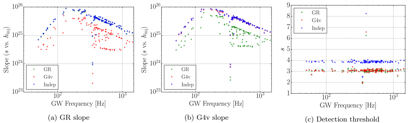
FIG. 10: Slope of the s vs. h_{\text{inj}} best-fit-line (left and center) and significance detection threshold at \alpha_n = 99.9\% (right) vs. GW frequency and for GR and G4v injections on S5 H1 data for 115 pulsars. Color corresponds to search template: GR, green; G4v, red; and model-independent, blue. Note that for both kinds of injections, the model-independent points overlap the matching template.
