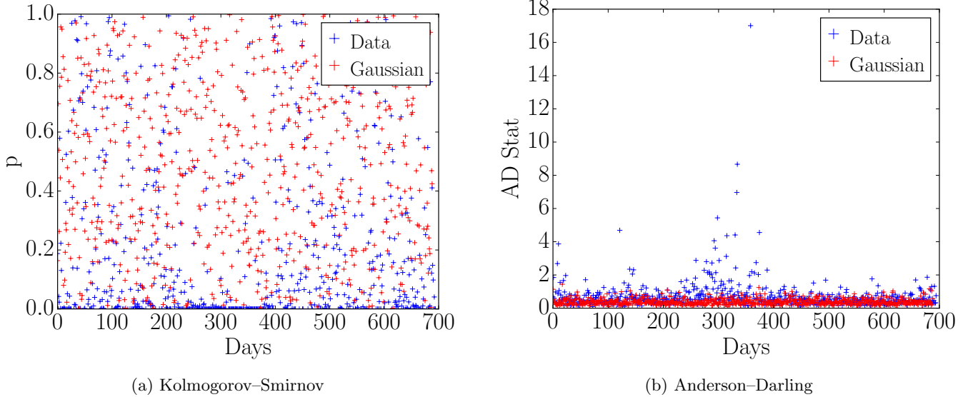
FIG. 15: Results of Gaussianity tests for daily segments of S5 H1 data prepared for the Crab (blue). The results for corresponding sets of Gaussian noise are presented for comparison (red).
