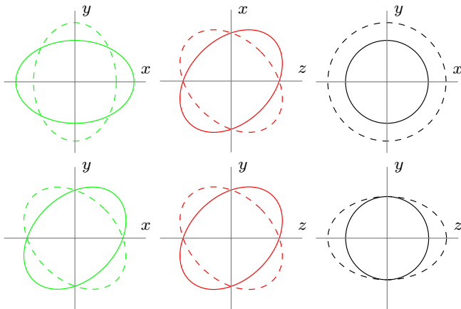
FIG. 1: Illustration of the effect of different GW polarizations on a ring of test particles. plus (+) and cross (x) tensor modes (green); vector-x (x) and vector-y (y) modes (red); breathing (b) and longitudinal (l) scalar modes (black). In all of these diagrams the wave propagates in the z -direction [1].
