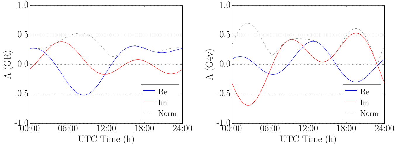
FIG. 3: Simulated GR (left) and G4v (right) heterodyned Crab signals as seen by LHO. The templates are generated from eq. (37) with the model parameters given in eqs. (5–8) and setting h_0 = 1 , \phi_0 = 0 . The solid curves represent the real (blue) and imaginary (red) parts, while the dashed curve corresponds to the complex norm.
