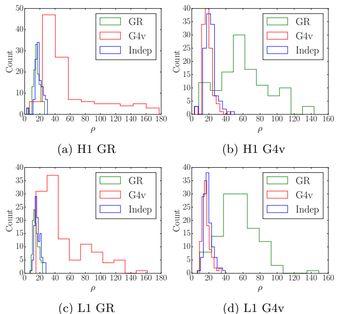
FIG. 13: Histograms of the figure of merit \rho , eq. (56), for our searches over S5 H1 (top) and L1 (bottom) data sets with GR (left) and G4v (right) injections, corresponding to 115 pulsars. Color corresponds to search template: GR, green; G4v, red; and model-independent, blue.
