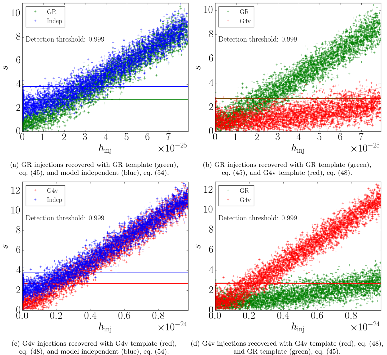
FIG. 9: GR (top) and G4v (bottom) injection results of search over LIGO S5 H1 data heterodyned for the Crab pulsar. Plots show significance, eq. (42), vs. injected strength. Color corresponds to the template used for recovery: GR, green; G4v, red; model-independent, blue. This particular search was performed using 10^4 instantiations, half of which contained injections using the values of \iota and \psi given in table I. The model-dependent templates assumed the same \iota as the injections. Horizontal lines correspond to a detection threshold \alpha_n = 99.9\% .
