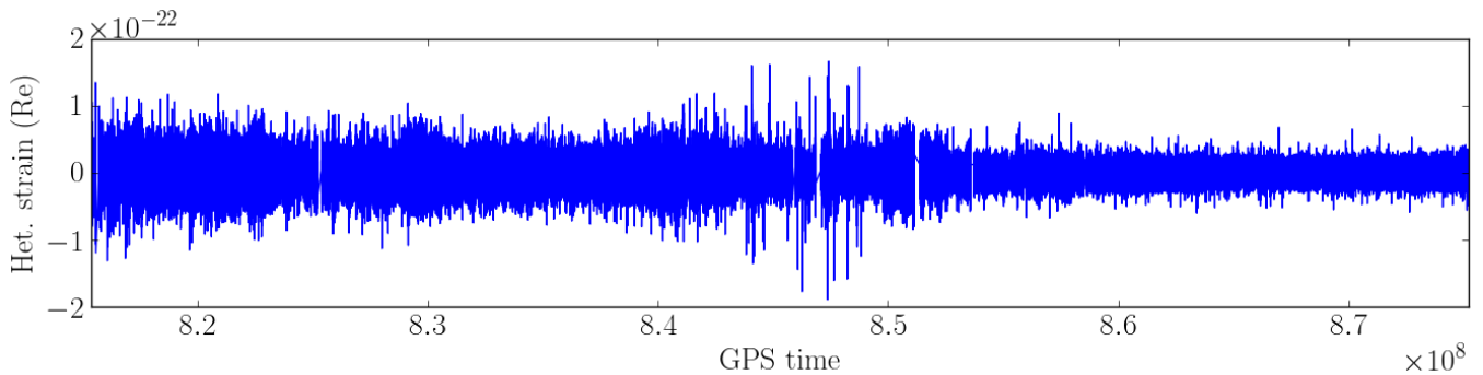
FIG. 4: Real part of LIGO Science Run 5 Hanford 4km detector (H1) minute-sampled data prepared for the Crab spanning approximately two years. A signal in these data would be described by eq. (39).
