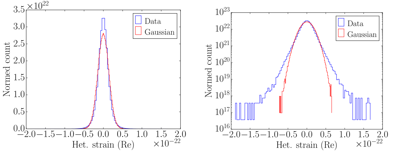
FIG. 14: Normalized histogram of the real part of S5 H1 data heterodyned for the Crab in linear (left) and logarithmic y scales. A Gaussian curve with the same standard deviation is plotted in red for comparison.
