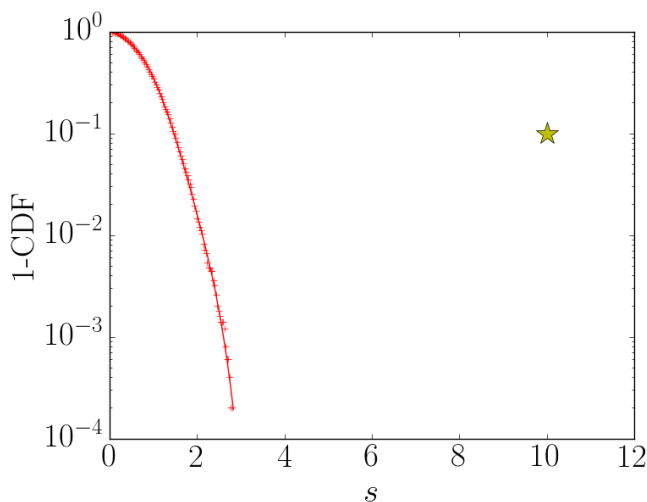
FIG. 7: Example plot of p = 1 - \text{CDF} vs. the recovery significance for a particular template. A loud injection in noise is manifested as an outlier (star) over the noise-only background (red). Note that the injection is plotted arbitrarily at p = 10^{-1} .
