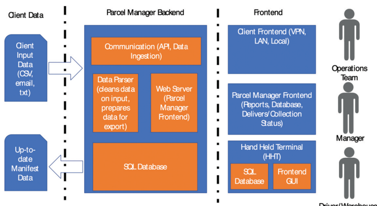
Menzies Distribution's IT system overview
