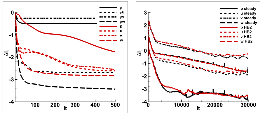
Fig. 6 Continuity and momentum residual convergence histories of TD COSA and ARCTIC at 60 of oscillation period (left), and steady and HB 2 ARCTIC analyses (right).
