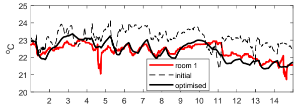
Fig. 1. Measured room temperatures for the first two weeks of September 2017 (axis: days), compared with the output of an electrical analogy model, for an illustrative room of the Charles Carter Building. The response of an initial model with physically-based coefficients (dashed) is compared to the response with coefficients that have been numerically optimised from measured data (solid).
