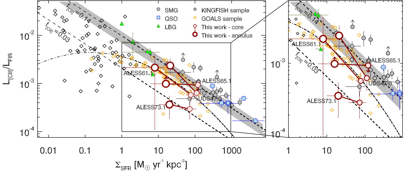
Figure 6. The L_{[\text{CII}]} to L_{\text{FIR}} ratio as a function of the star-formation rate density for local galaxies in the KINGFISH and GOALS (Armus et al. 2009; D\u00edaz-Santos et al. 2017; Lutz et al. 2016b), a sample of high-redshift galaxies (Wang et al. 2013; Kimball et al. 2015; Capak et al. 2015; Gullberg et al. 2015; D\u00edaz-Santos et al. 2017; Nesvadba et al. 2016; Umehata et al. 2017; Lutz et al. 2016a; Jones et al. 2017; Venemans et al. 2017), and our sample of four z \sim 4.5 SMGs. We note that the sizes used to achieve the star-formation rate densities for the GOALS sample are the 70\mu\text{m} effective radii under the assumption of a uniform dust temperature. The inner parts of our four galaxies are plotted as red-circles and the outer annuli as stars. The respective core and annuli measurements are connected by solid lines. For three SMGs in the sample the \Sigma_{\text{SFR}} is lower in the outer annulus and the L_{[\text{CII}]} / L_{\text{FIR}} ratios is higher than for the core. This suggests that the [CII] deficit is a local process. The L_{[\text{CII}]} / L_{\text{FIR}} ratio as a function of the FIR surface density and the mass fraction of [CII] compared to the total mass ( f_{[\text{CII}]} ) from Mu\u00f1oz & Oh (2016) is plotted as the gray shaded area, assuming f_{[\text{CII}]} = 0.10 - 0.17 , and the curved power law fitted to galaxies in GOALS from (D\u00edaz-Santos et al. 2017) is plotted as the dot-dashed curve. We note that both the high and low redshift samples exhibit a large scatter around the two models. Our data agrees with both models and so it is not possible to distinguish which of the two models is closer to the true explanation.
