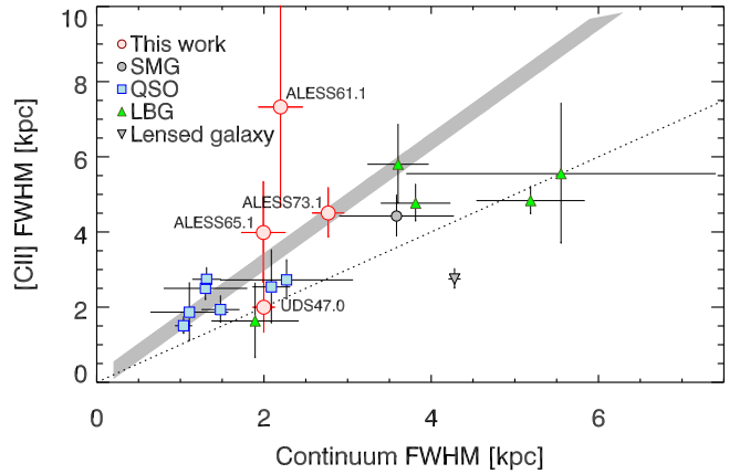
Figure 4. Spatial FWHM of the rest frame 160\ \mu\text{m} continuum emission versus the FWHM of the [CII] emission for the four SMGs in this work and high-redshift ( 3.1 < z < 7.1 ) galaxies in the literature with similar measurements (Wang et al. 2013; Capak et al. 2015; Kimball et al. 2015; Nesvadba et al. 2016; Umehata et al. 2017; Díaz-Santos et al. 2016; Venemans et al. 2017; Jones et al. 2017). We see that the [CII] emitting gas is more extended than the rest frame 160\ \mu\text{m} emitting dust for the majority of the galaxies. The dotted line is the 1:1 relation, while the gray shaded region shows the weighted mean of the [CII] to continuum size of 1.6 \pm 0.4 .
