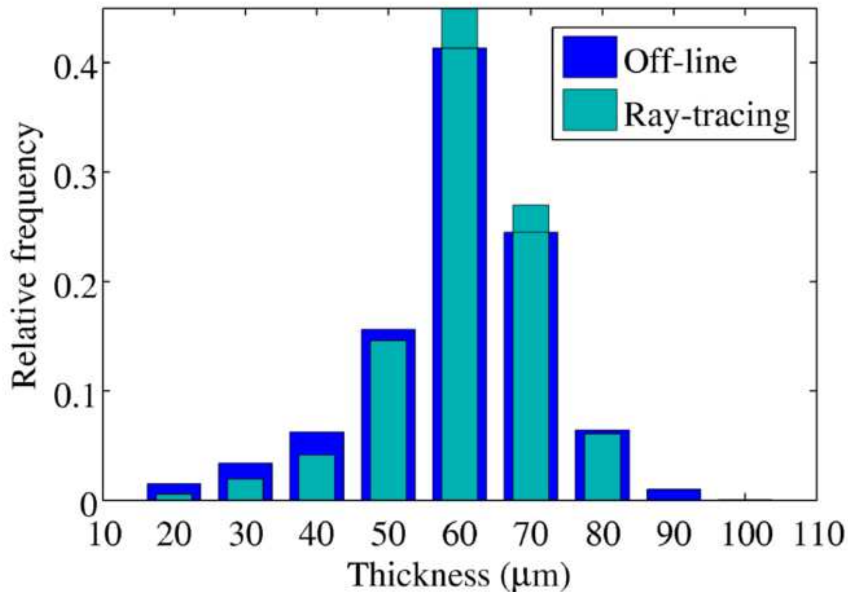
(c) 6 baffles
