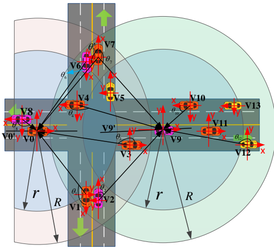
Fig. 4. A schematic diagram of message propagation in the proposed protocol.
