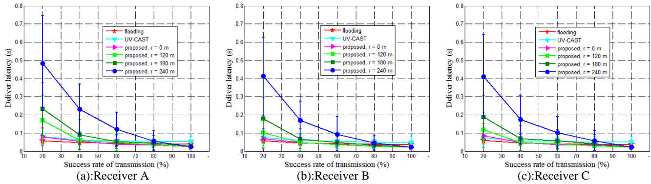
Fig. 9. The deliver latency under each protocol with different transmission conditions observed at the receiver A, B and C, respectively.(a) Observed at receiver A. (b) Observed at receiver B. (c) Observed at receiver C.
