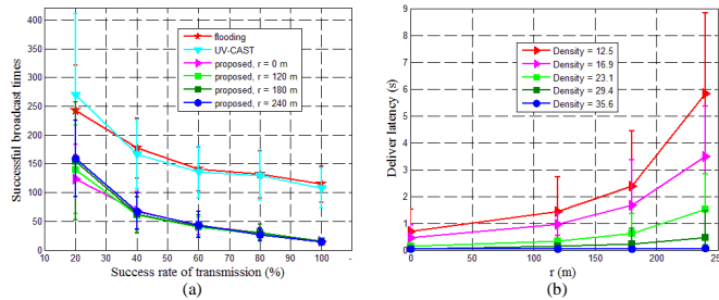
Fig. 11. (a) The total times that forwarders broadcasted the message successfully during the simulation time under different protocols with different transmission conditions. (b) The deliver latency observed at the receiver A under different r with different traffic flow densities, and p was set to be 0.6 in the simulation.
