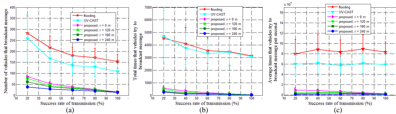
Fig. 10. (a) The number of vehicles that have taken part in broadcasting message during the simulation time. (b) The total times that vehicles tried to broadcast message under each protocol with different transmission conditions during the simulation time. (c) The average times that vehicles tried to broadcast message per second under the three protocols with different transmission conditions.
