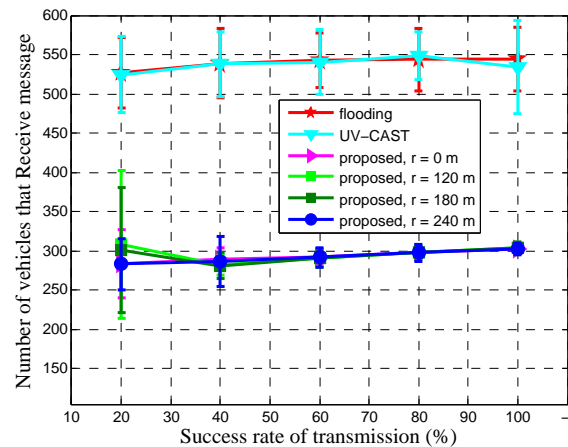
Fig. 8. The number of vehicles that have received message during the simulation time under different protocols with different transmission conditions.
