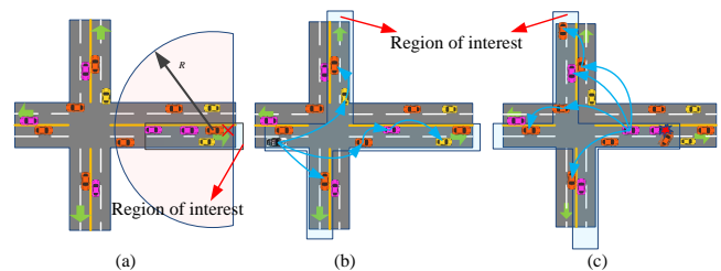
Fig. 2. Schematic diagram of different types of messages' region of interest. (a)Region of interest of one-hop broadcasted messages typed by "0"; (b)Region of interest of forward multi-hop broadcasted messages typed by "1"; (c)Region of interest of backward multi-hop broadcasted messages typed by "2".
