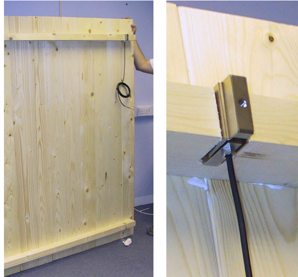
Fig. 4. The floor when it was installed in upright position (left). Enlarged view of the load cell embedded into the floor (right).
