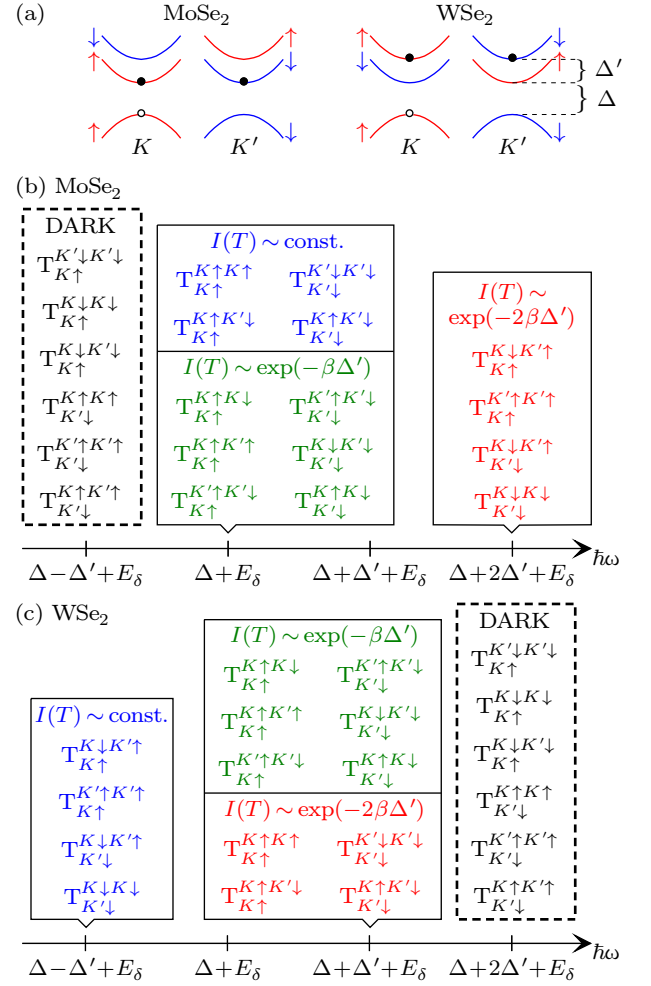
FIG. 2. (Color online) As Fig. 1, but for negative triions in molybdenum and tungsten dichalcogenides. E' δ ≡ E X - is the total energy E X - of a negative triion. T k 1 σ 1 k 2 σ 2 k 3 σ 3 denotes a triion consisting of conduction-band electrons in valleys k 1 and k 2 with spins σ 1 and σ 2 and a valence-band hole in valley k 3 with spin σ 3 .
