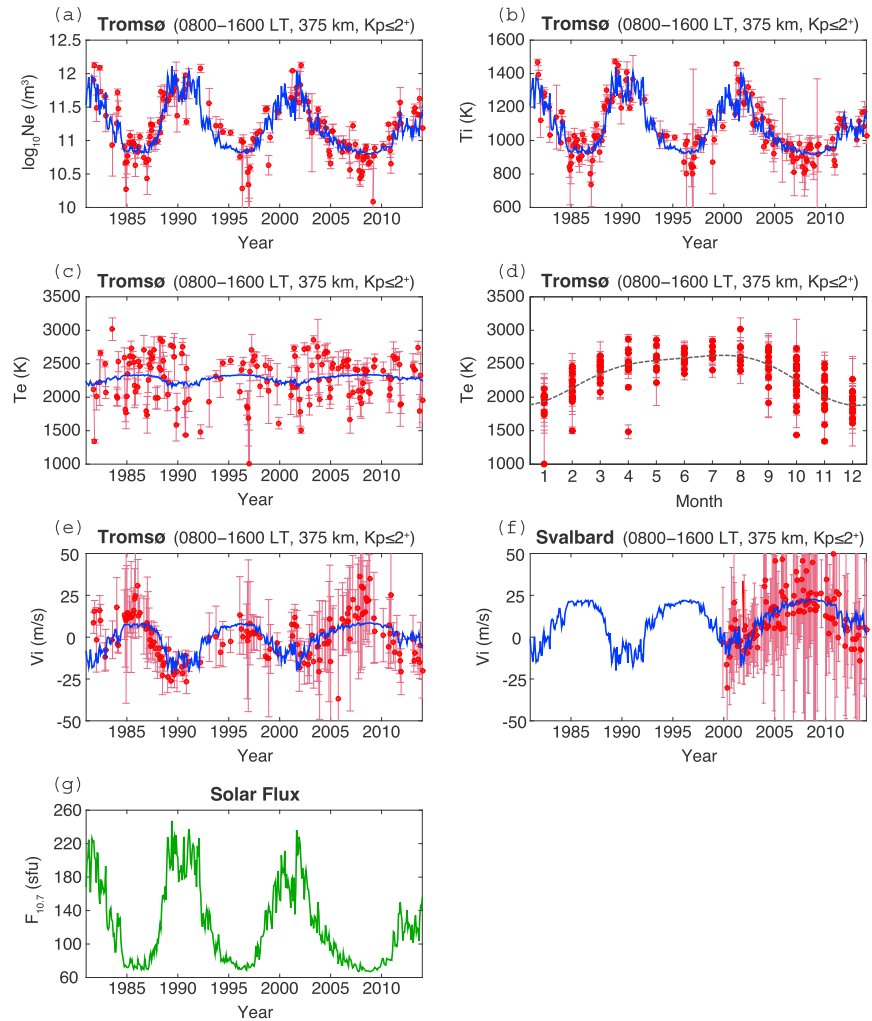
Figure 1. Time series of (a) plasma density ( N_e ), (b) ion temperature ( T_i ), (c) electron temperature ( T_e ), and (e) field-aligned ion velocity ( \mathbf{V}_{\parallel} , positive upward) at 375 km, obtained from the EISCAT radar at Tromsø under geomagnetically quiet conditions ( K_p \leq 2^+ ) during 1981–2014. Shown are monthly averages of the daytime measurements (0800–1600 LT). The error bars represent the standard deviation, and the blue lines represent the least squares fit of the function C = a + bF_{10.7} to the corresponding ionospheric data (see text for details). (d) Seasonal variation of T_e , with the least squares fit of the function D = \sum_{k=0}^2 \{a_k \cos(kM/12) + b_k \sin(kM/12)\} (see text for details). (f) Same as Figure 1e except for Svalbard. (g) Monthly values of the F_{10.7} index.
