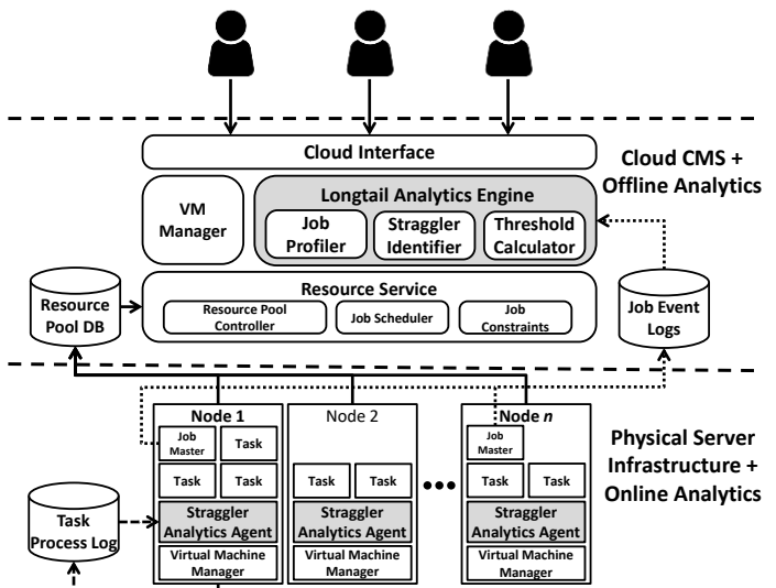
Fig 7. Cloud datacenter model with integrated Long Tail analytics engine and agent based analytics.
