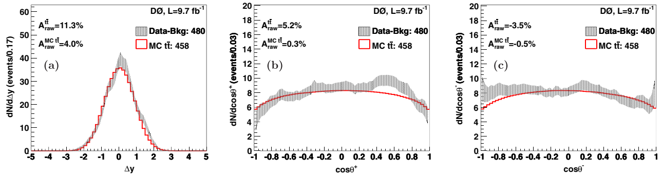
FIG. 3 (color online). Estimated distribution of the (a) \Delta y_{i\bar{i}} , (b) \cos \theta^+ , and (c) \cos \theta^- observables in dilepton events after subtracting the expected background contribution. Deviations between the background-subtracted data and MC can be attributed to statistical fluctuations. The background-subtracted data asymmetries and the MC asymmetries extracted from these distributions are also reported. These raw asymmetries need to be corrected for calibration effects to retrieve the parton-level asymmetries.
