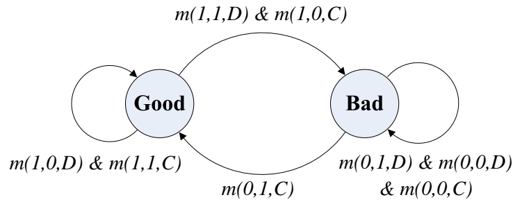
Figure 3.1: The 8 reputation transitions of BioTrust
