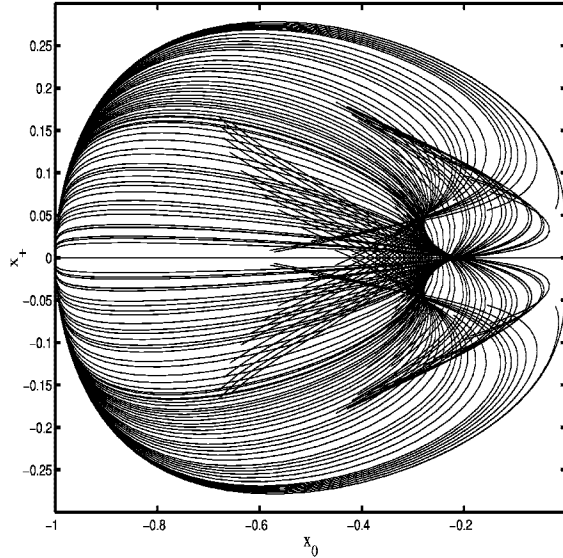
FIGURE 2. Optimal trajectories for \Gamma = 0.3
