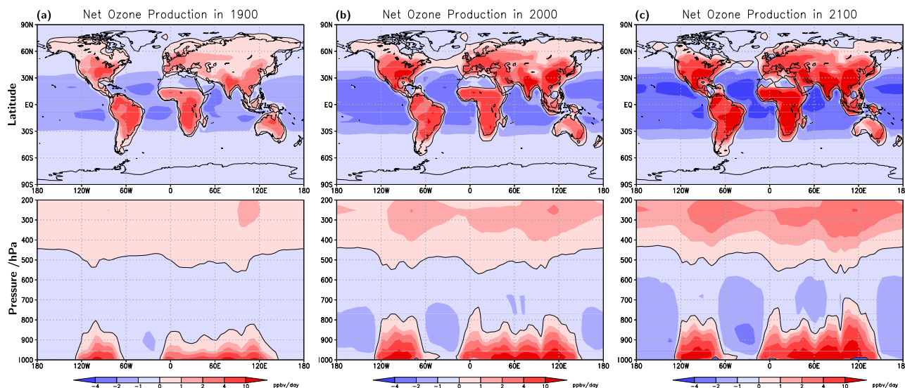
Figure 1. Annual mean distribution of net O_3 production in ppbv/day in (top) the boundary layer and (bottom) at northern mid-latitudes (20–60°N) in (a) 1900, (b) 2000, and (c) 2100. The contour line marks zero net production.
