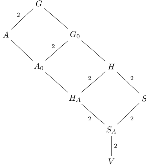
Figure 3. Subgroups of \Sigma_{2p+1} .
