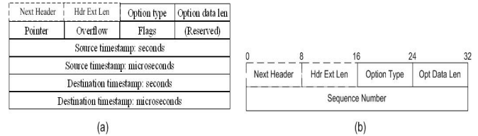
Figure 1. (a) One-Way Delay and (b) One-Way Loss Measurement Destination Options Headers
